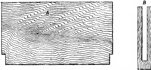
Fig. 14.—A, Inner walls of Doubling-box, showing slot which slides in the grooved pieces of wood (B), nailed to outer walls.
