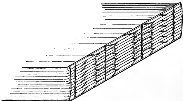
FIGURE 4.—Old-fashioned whipstitching. Each section is sewed separately.
