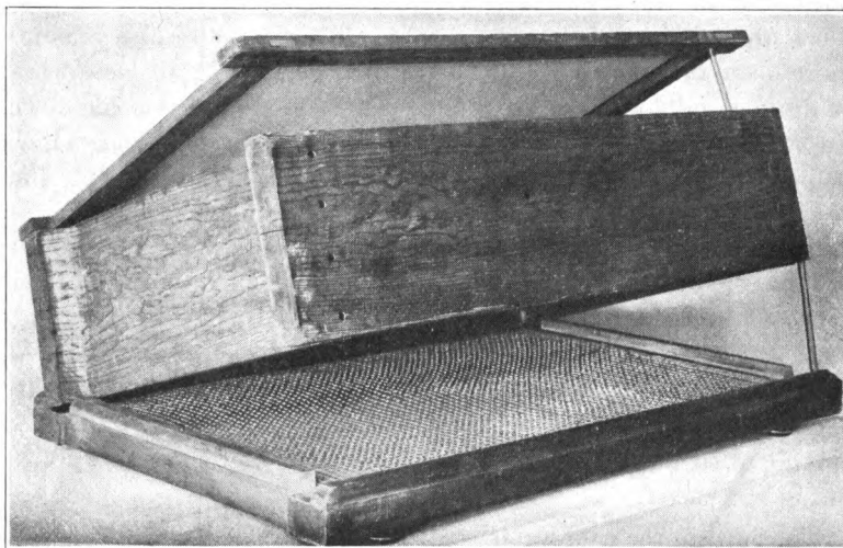
FIG. 1. A DRAINING RACK SUITABLE FOR A LARGE CREAMERY The rack is shown with the front side raised so that the three essential parts may be seen.
