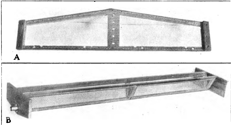
FIG. 4. WIRE NETTING ON A FRAME MAKES A CONVENIENT STRAINER Either the strainer which fits across the bottom of the vat (A) or the trough strainer (B) may be used to supplement the cylindrical vat strainer in draining a large mass of curd.
