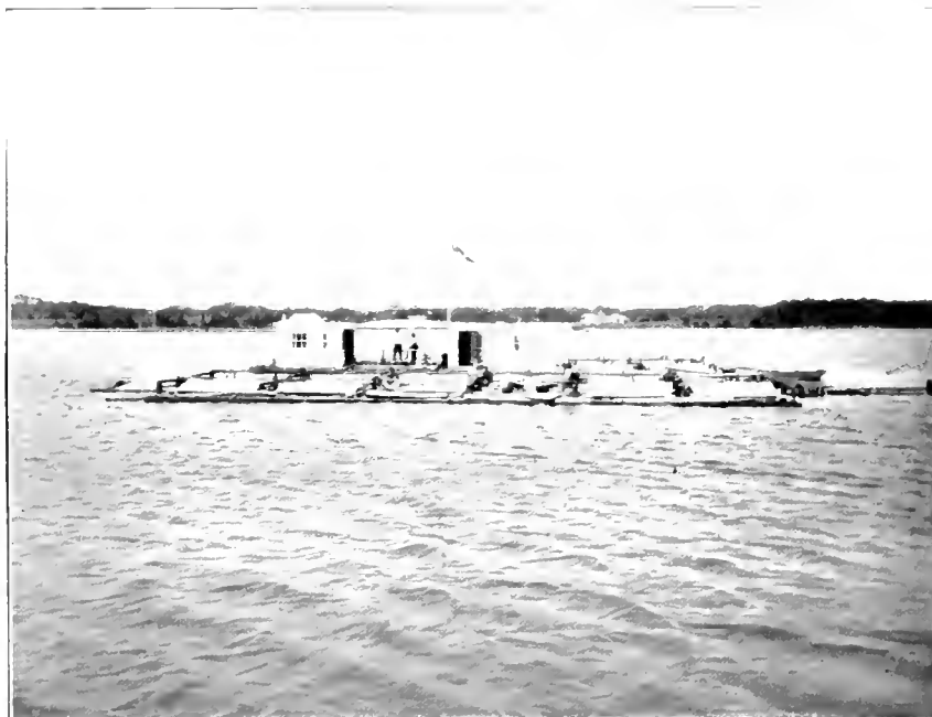
FIG. 1.—Floating laboratory and rearing plant from the port side. The forward deck house serves as a laboratory and the after one as the engine house and tool room. Most of the rearing cars are covered with white awnings.
