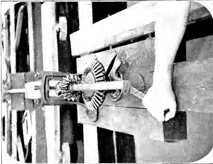
FIG. 21.—Detail of device for throwing propeller in and out of gear. By pushing the lever the propeller shaft and its gear drop as in fig. 22.
