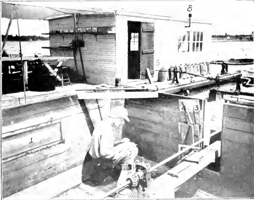
FIG. 11. Interior of rearing car. Preparing to caulk small cracks before lowering the car. 1, side window; 2, end slot; 3, doors for same; 4, buttons to hold doors shut; 5 and 6, the transverse shaft, universal joint, and sliding sleeve; 8, exhaust and muffler.
