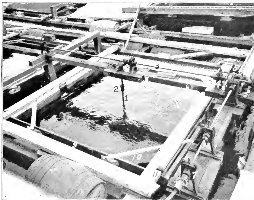
FIG. 8.—Car with propeller in motion. From propeller the shafting may be followed back (1, 2) to the universal joint—1, propeller shaft; 2, sleeve coupling; 3, longitudinal shaft; 4, adjustable shaft hanger; 5, gear trains from longitudinal to transverse shafts; 6, transverse horizontal shaft of float; 7, shaft hanger; 8, ball joint connecting shaft with that of house boat; 9, edge of rearing box; 10, brace across corner of rearing box; 11, holding-down plank mortised into corner post; 12, shaft beam.
