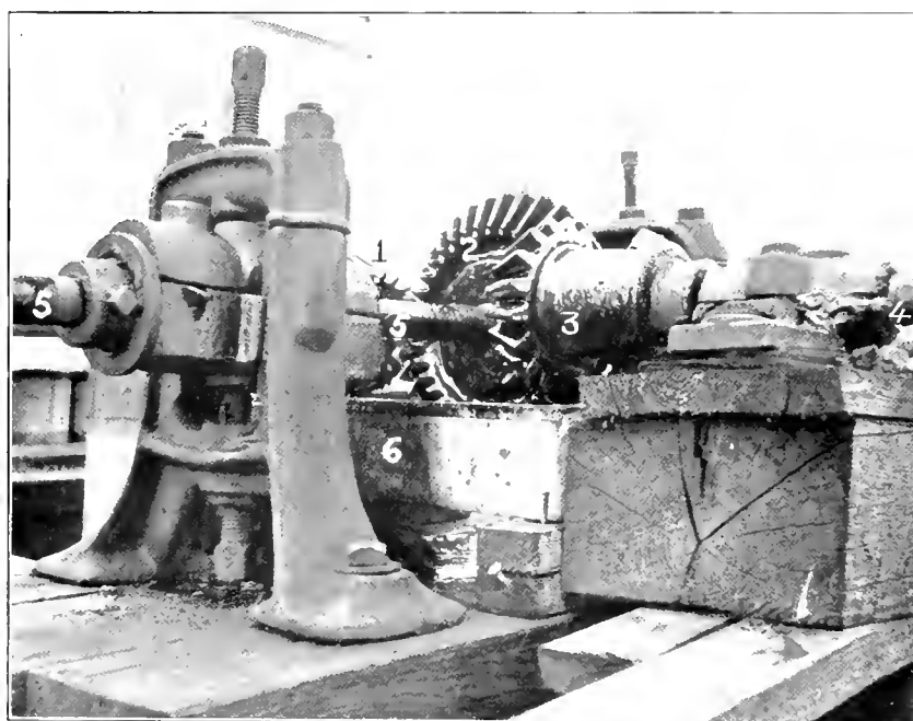
FIG. 20. Detail of gears on float at junction of transverse and longitudinal shafts. (Compare fig. 4, pl. XCII.) 1, gear on horizontal shaft from house boat; 2, large gear on longitudinal shaft, reducing speed one-half; 3, gear on the inner end of transverse shaft (4); 4, shaft transmitting power to outer float; 5, longitudinal shaft on inner float; 6, oil box.
