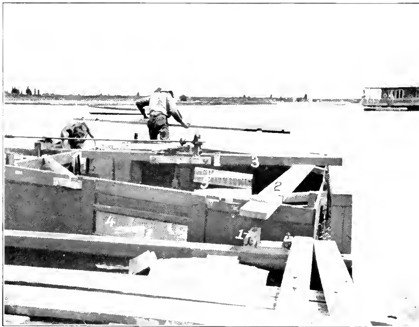
FIG. 10.—The cleats being removed, the car rises part way by its own buoyancy. Opening doors of the slot at end of car to admit the longitudinal shaft beam allows the car to be entirely raised. 1, cleat, 2, holding-down plank, 3, longitudinal shaft beam, 4 and 5, side windows.
