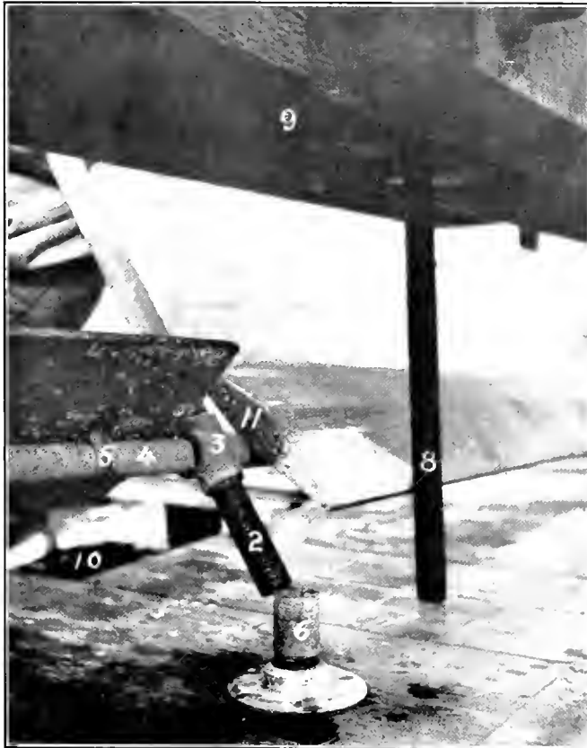
FIG. 18.—Detail of lower portion of the propeller shaft and its socket in floor of car. 1, propeller shaft, made of gas pipe; 2, short portion of shaft made of steel, to fit into the socket (6); 3, four-way pipe coupling; 4, gas pipe to which blades are strapped; 5, strap holding propeller blades; 6 and 7, socket and flange; 8, upper disconnected steel portion of the propeller shaft; 9, shaft beam; 10, window in bottom of car; 11, base of propeller blade, showing in section the shape.
