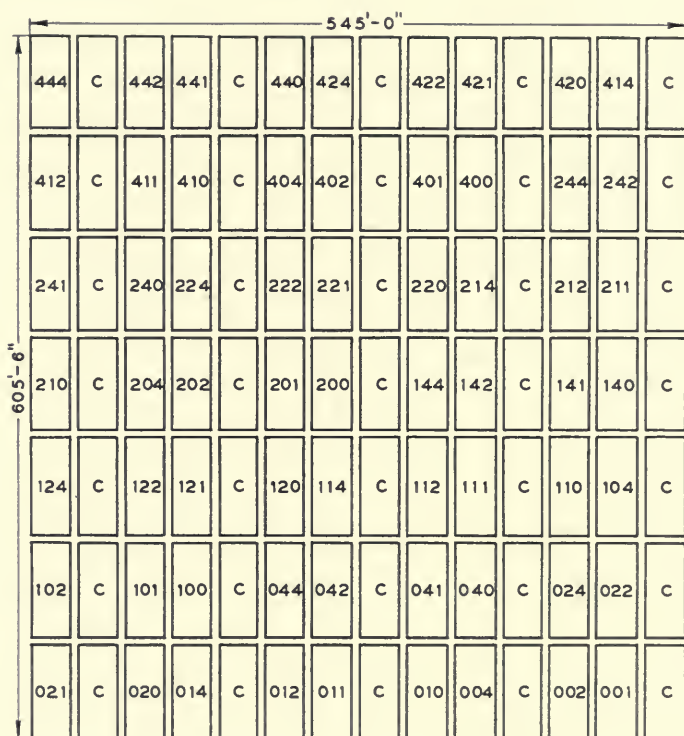
FIG. 1.—PLOT ARRANGEMENT IN FIELD 800
