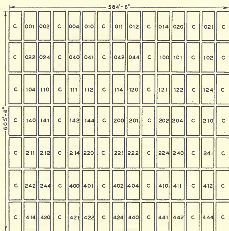
FIG. 3.—PLOT ARRANGEMENT IN FIELD 1000
