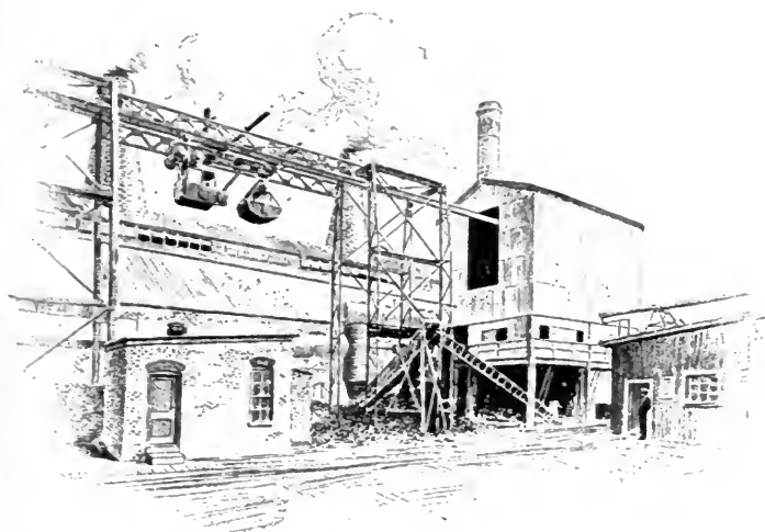
Part of Gas Producer Plant at the Charleroi Works
