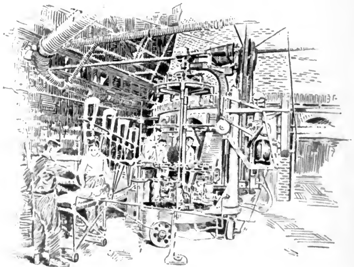
Making Lamp Chimneys with Machine
