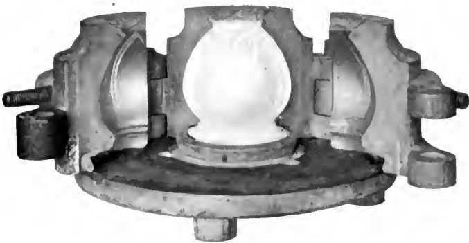
Iron Blow Mold
