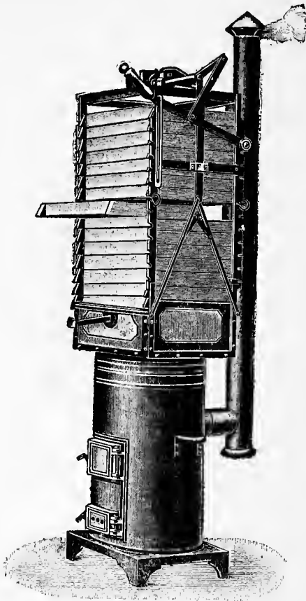
THE LARGER EVAPORATOR
