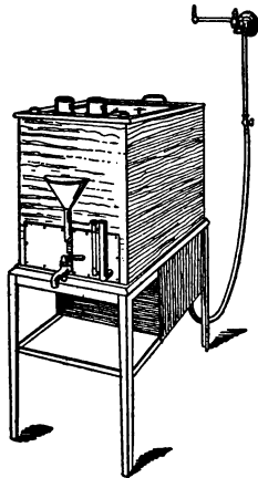
FIG. 61.—Incubator.
