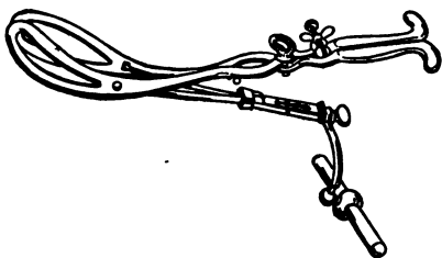
FIG. 42.—Tarnier's axis-traction forceps.
