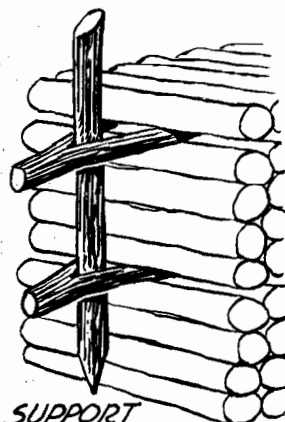
SUPPORT FOR PULPWOOD ON FROZEN GROUND
