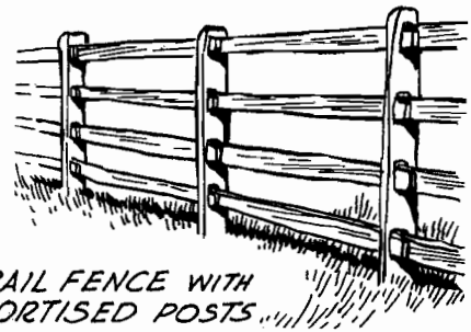
RAIL-AND-STAKE FENCE
