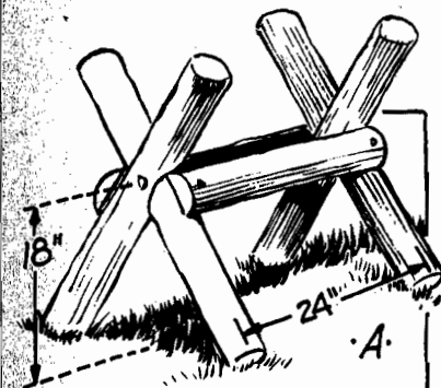
SAWBUCKS FOR SMALL STUFF
