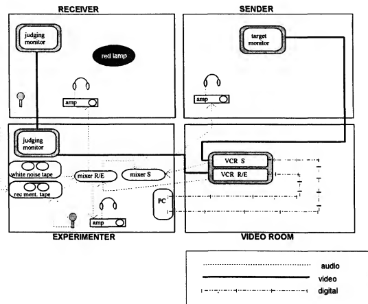
Figure 2. Audio, video, and digital communications layout. This design isolates the audio and video (a/v) paths for the sender and the receiver/experimenter to avoid introducing sensory cues. The only direct connection between the sender's and the receiver's a/v systems is the output of the audio mixer into the input of the sender's audio mixer.
