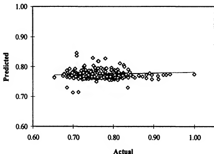
Figure 19. Correlation between abductive network's predictions of casino payout rates and actual payout rates for scrambled data; r = 0.0346 , t = 0.583 , 353 df , p = 0.561 .
