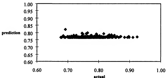
Figure 17. Correlation between neural network's predictions of casino payout rates and actual payout rates for the scrambled data; r = -0.012 , t = -0.200 , 282 df , p = 0.841 . The variance in the control output shown here is restricted because the neural network defaults to a 'best-guess' output when it cannot learn meaningful relationships between the inputs and output.
