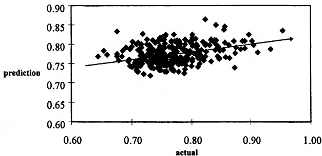
Figure 16. Correlation between neural network's predictions of casino payout rates and actual payout rates; N = 284 , r = 0.32 , t = 5.74 , 282 df, p < 0.001 .
