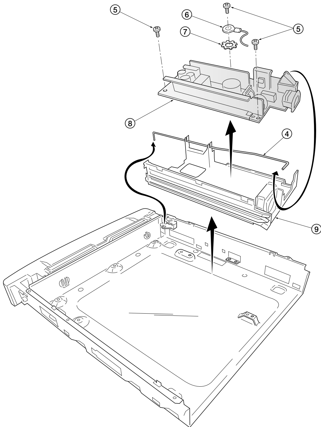
Figure 5-2-20 Removing the power supply unit
