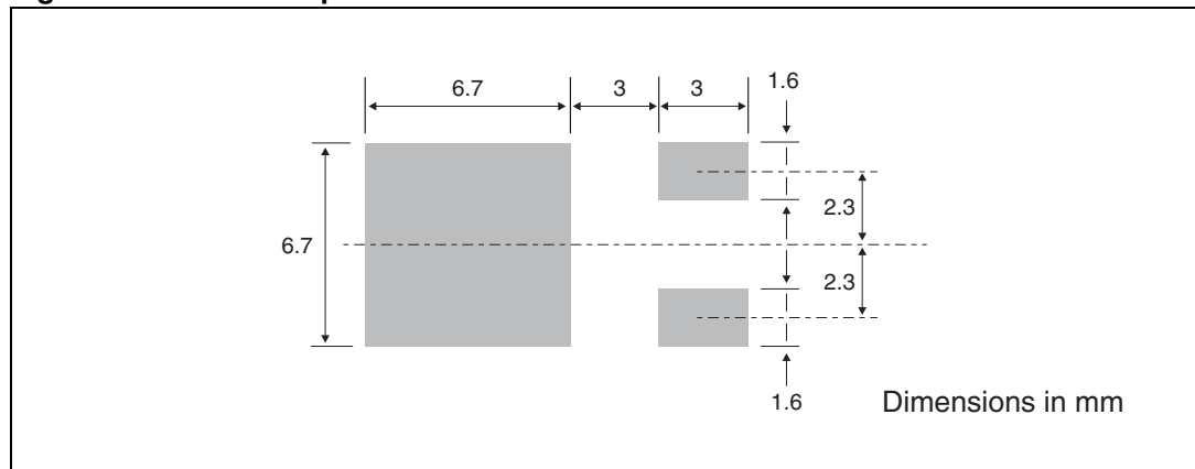
Figure 19. DPAK footprint
