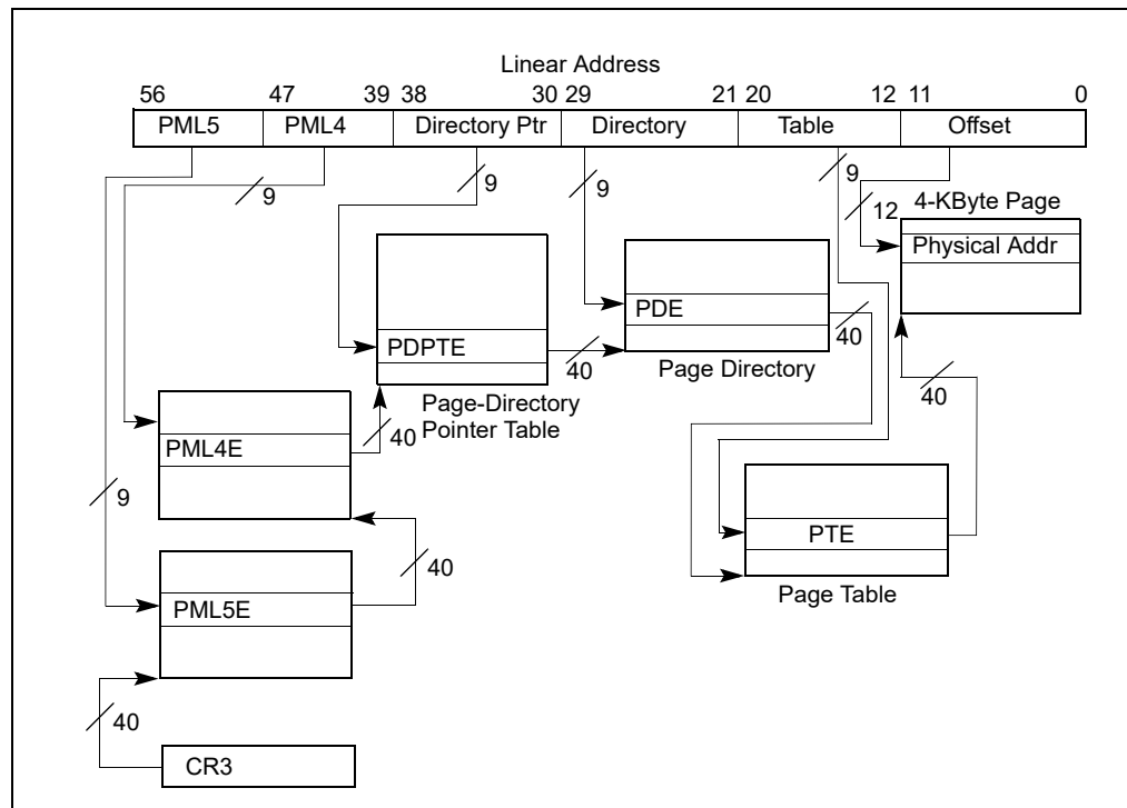
Figure 2-1. Linear-Address Translation Using 5-Level Paging
