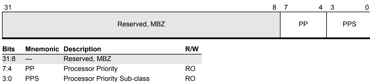
Figure 16-27. Processor Priority Register (APIC Offset A0h)
