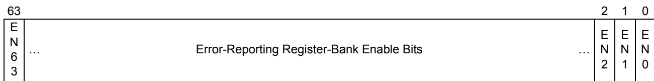
Figure 9-5. MCi\_CTL Register
