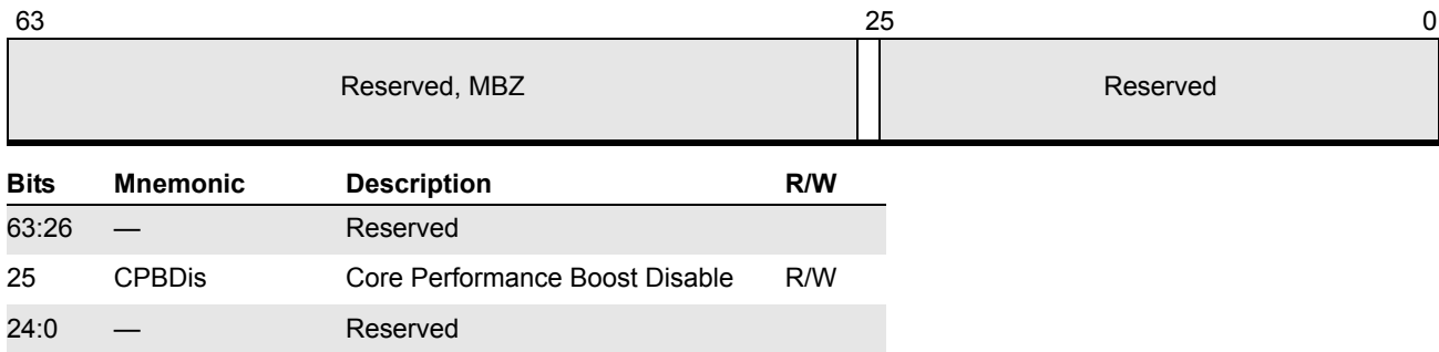
Figure 17-4. Core Performance Boost (MSRC001_0015h)
