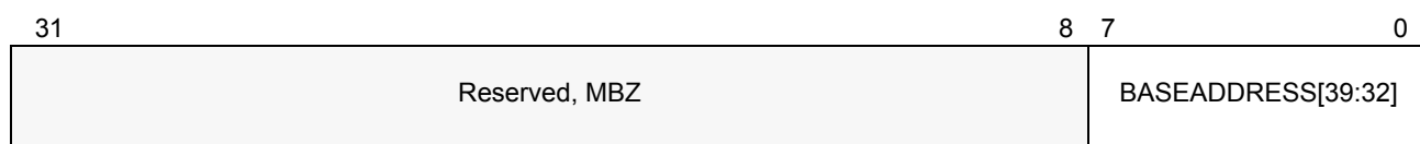
Figure 15-9. Format of DEV_BASE_HI[n] Registers
