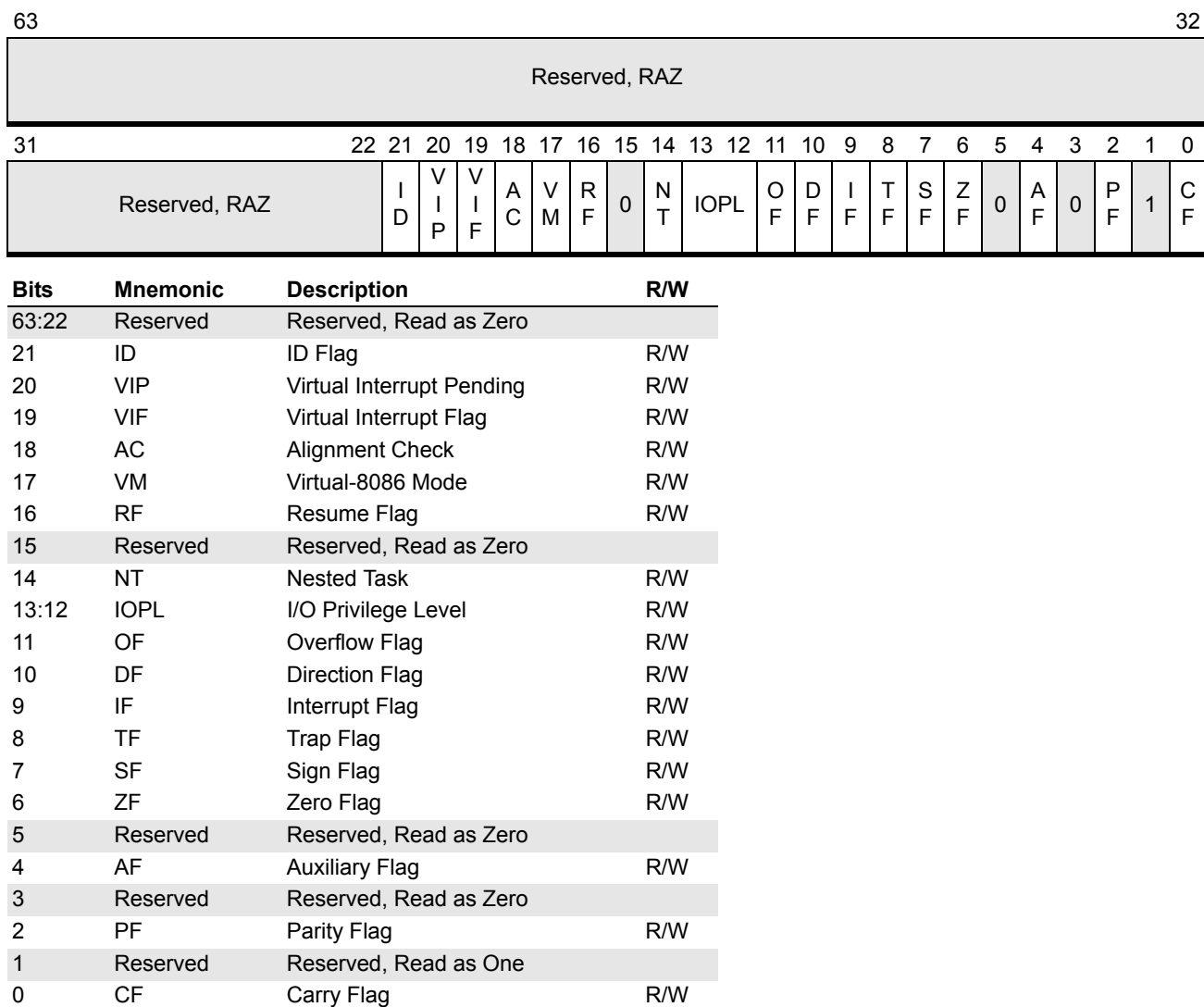
Figure 3-8. RFLAGS Register
