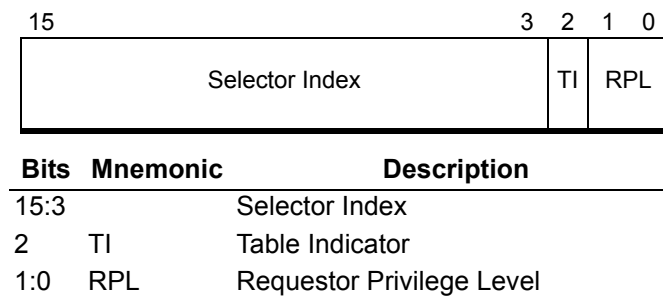
Figure 12-2. Task-Segment Selector
