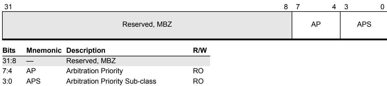
Figure 16-22. Arbitration Priority Register (APIC Offset 90h)
