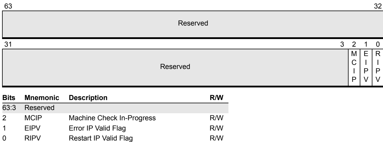
Figure 9-2. MCG_STATUS Register
