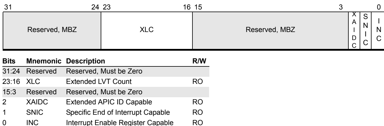
Figure 16-5. Extended APIC Feature Register (APIC Offset 400h)
