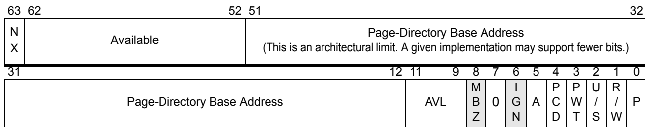
Figure 5-24. 2-Mbyte PDPE—Long Mode
