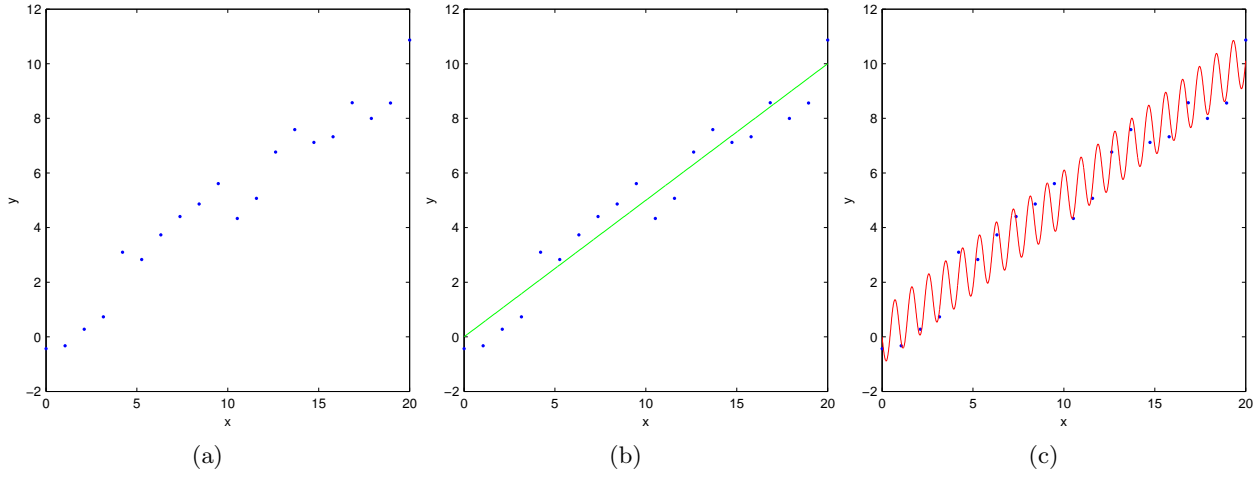
Figure 12.6: (a) : Data for which we wish to fit a regression model. (b) : The best ‘simple’ model fit y = ax has maximum likelihood 5.9 \times 10^{-11} . (c) : The best ‘complex’ model fit y = ax + \cos(bx) has maximum likelihood 1.1 \times 10^{-10} .
