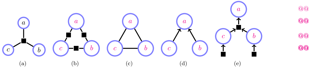
Figure 4.8: (a) : \phi(a, b, c) . (b) : \phi(a, b)\phi(b, c)\phi(c, a) . (c) : \phi(a, b, c) . Both (a) and (b) have the same undirected graphical model, (c). (d) : (a) is an undirected FG of (d). (e) : Directed FG of the BN in (d). A directed factor represents a term p(\text{children}|\text{parents}) . The advantage of (e) over (a) is that information regarding the marginal independence of variables b and c is clear from graph (e), whereas one could only ascertain this by examination of the numerical entries of the factors in graph (a).
