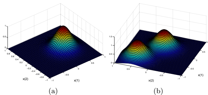
Figure 17.6: (a): The output of an RBF function \exp(-\frac{1}{2}(\mathbf{x} - \mathbf{m}^1)^2/\alpha^2) . Here \mathbf{m}^1 = (0, 0.3)^\top and \alpha = 0.25 . (b): The combined output for two RBFs with \mathbf{m}^1 as above and \mathbf{m}^2 = (0.5, -0.5)^\top .
