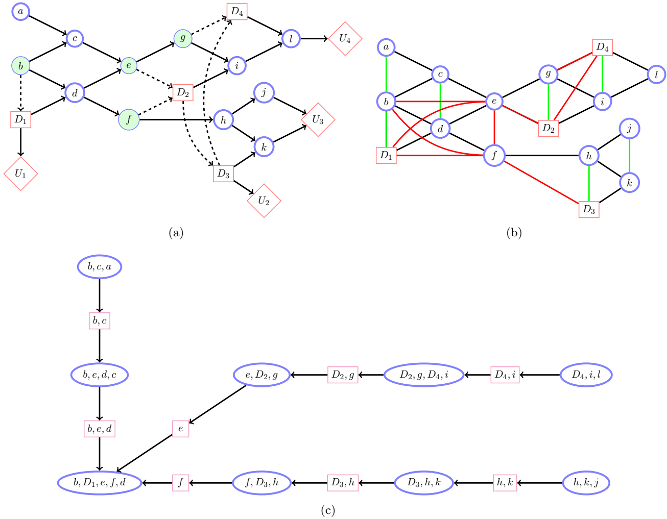
Figure 7.7: (a): Influence Diagram, adapted from [159]. Causal consistency is satisfied since there is a directed path linking all decisions in sequence. The partial ordering is b \prec D_1 \prec (e, f) \prec D_2 \prec (\cdot) \prec D_3 \prec g \prec D_4 \prec (a, c, d, h, i, j, k, l) . (b): Moralised and strongly triangulated graph. Moralisation links are in green, strong triangulation links are in red. (c): Strong Junction Tree. Absorption passes information from the leaves of the tree towards the root.
