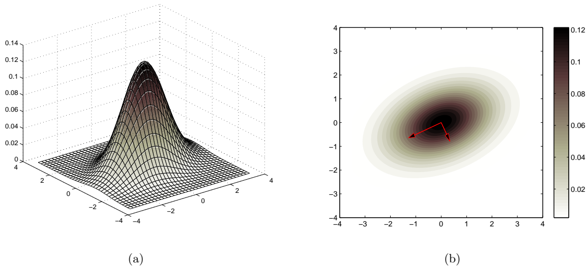
Figure 8.7: (a): Bivariate Gaussian with mean (0, 0) and covariance [1, 0.5; 0.5, 1.75] . Plotted on the vertical axis is the probability density value p(x) . (b): Probability density contours for the same bivariate Gaussian. Plotted are the unit eigenvectors scaled by the square root of their eigenvalues, \sqrt{\lambda_i} .
