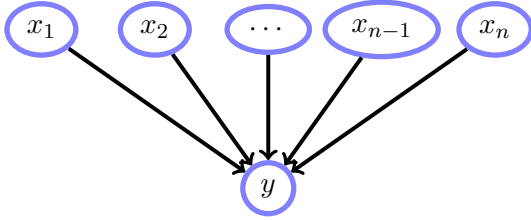
Figure 9.7: A variable y with a large number of parents x_1, \dots, x_n requires the specification of an exponentially large number of entries in the conditional probability p(y|x_1, \dots, x_n) . One solution to this difficulty is to parameterise the conditional, p(y|x_1, \dots, x_n, \theta) .
