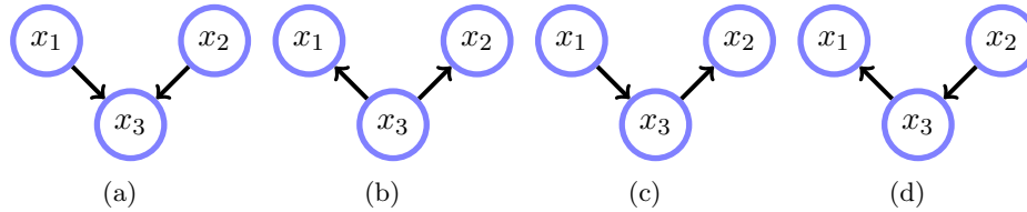
Figure 3.6: By dropping say the connection between variables x_1 and x_2 , we reduce the 6 possible BN graphs amongst three variables to 4. (The 6 fully connected ‘cascade’ graphs correspond to (a) with x_1 \rightarrow x_2 , (a) with x_2 \rightarrow x_1 , (b) with x_1 \rightarrow x_2 , (b) with x_2 \rightarrow x_1 , (c) with x_1 \rightarrow x_2 and (d) with x_2 \rightarrow x_1 . Any other graphs would be cyclic and therefore not distributions).
