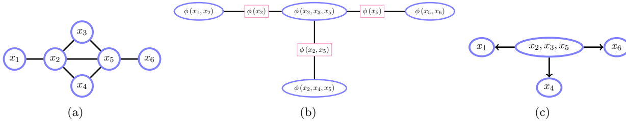
Figure 9.16: (a): A decomposable Markov network. (b): A junction tree for (a). (c): Set chain for (a) formed by choosing clique x_2, x_3, x_5 as root and orienting edges consistently away from the root. Each separator is absorbed into its child clique to form the set chain.
