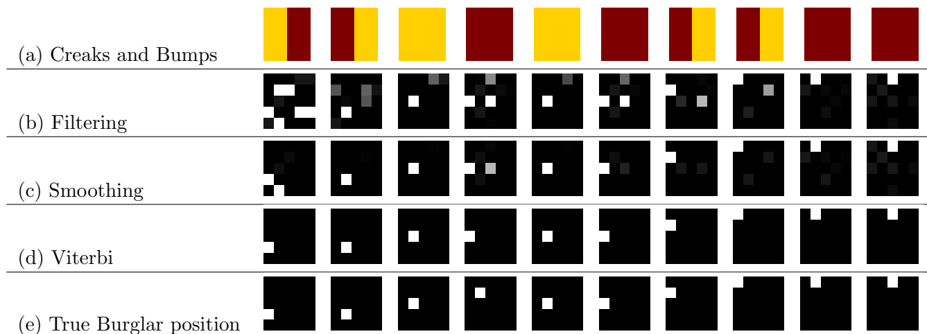
Figure 23.6: Localising the burglar. The latent variable h_t \in \{1, \dots, 25\} denotes the positions, defined over the 5 \times 5 grid of the ground floor of the house. (a): A representation of the probability that the ‘floor will creak’ at each of the 25 positions, p(v^{creak}|h) . Light squares represent probability 0.9 and dark square 0.1. (b): A representation of the probability p(v^{bump}|h) that the burglar will bump into something in each of the 25 positions.
