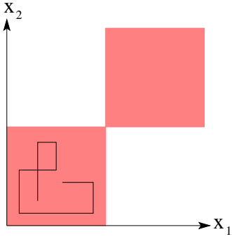
Figure 27.5: A two dimensional distribution for which Gibbs sampling fails. The distribution has mass only in the shaded quadrants. Gibbs sampling proceeds from the l^{\text{th}} sample state (x_1^l, x_2^l) and then sampling from p(x_2|x_1^l) , which we write (x_1^{l+1}, x_2^{l+1}) where x_1^{l+1} = x_1^l . One then continues with a sample from p(x_1|x_2 = x_2^{l+1}) , etc. If we start in the lower left quadrant and proceed this way, the upper right region is never explored.
