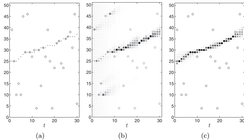
Figure 23.9: Filtering and smoothing for robot tracking using an HMM with S = 50 . (a) : A realisation from the HMM example described in the text. The dots indicate the true latent locations of the robot, whilst the open circles indicate the noisy measured locations. (b) : The squares indicate the filtering distribution at each timestep t , p(h_t | v_{1:t}) . This probability is proportional to the grey level with black corresponding to 1 and white to 0. Note that the posterior for the first timesteps is multimodal, therefore the true position cannot be accurately estimated. (c) : The squares indicate the smoothing distribution at each timestep t , p(t | v_{1:T}) . Note that, for t < T , we estimate the position retrospectively and the uncertainty is significantly lower when compared to the filtered estimates.
