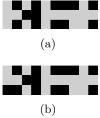
Figure 26.7: (a): The training sequence consists of a random set of vectors ( V = 3 ) over T = 10 time steps. (b): The reconstruction using H = 7 hidden units. The initial state \mathbf{v}(t = 1) for the recalled sequence was set to the correct initial training value albeit with one of the values flipped. Note that the method is capable of sequence disambiguation in the sense that transitions of the form \mathbf{a}, \mathbf{b}, \dots, \mathbf{a}, \mathbf{c} can be recalled.
