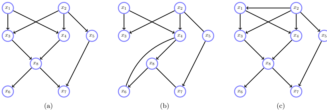
Figure 9.14: Learning the structure of a Bayesian network. (a): The correct structure in which all variables are binary. The ancestral order is x_2, x_1, x_5, x_4, x_3, x_8, x_7, x_6 . The dataset is formed from 1000 samples from this network. (b): The learned structure based on the PC algorithm using the Bayesian empirical conditional independence test. Undirected edges may be oriented arbitrarily (provided the graph remains acyclic). (c): The learned structure based on the Bayes Dirichlet network scoring method. See demoPCdata.m and demoBDscore.m .
