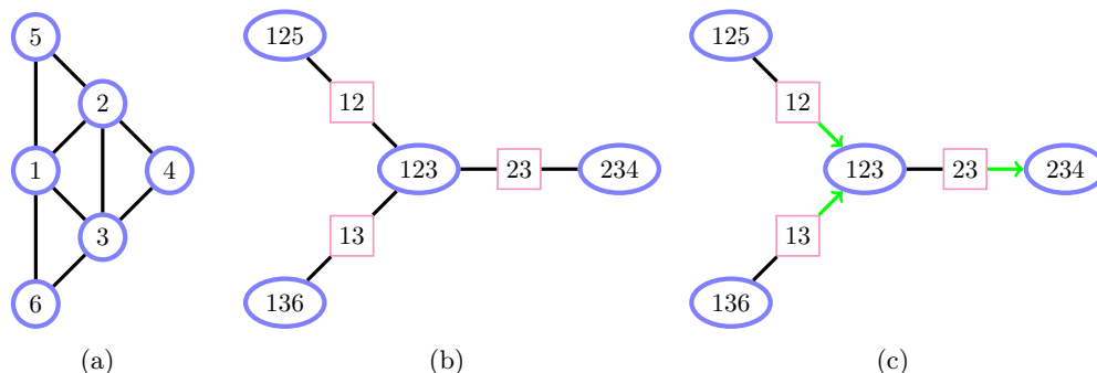
Figure 6.12: (a): Markov network. (b): Junction tree. Under absorption, once we have absorbed from 125 to 123 and 136 to 123, the result of these absorptions is stored in the new potential on 123. After this we can absorb from 123 to 234 by operating on the 123 potential and then sending this information to 234. (c): In Shafer-Shenoy updating, we send a message from a clique to a neighbouring clique based on the product of all incoming messages.
