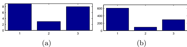
Figure 27.2: Histograms of the samples from the three state distribution p(x) = \{0.6, 0.1, 0.3\} . (a) : 20 samples. (b) : 1000 samples. As the number of samples increases, the relative frequency of the samples tends to the distribution p(x) .
