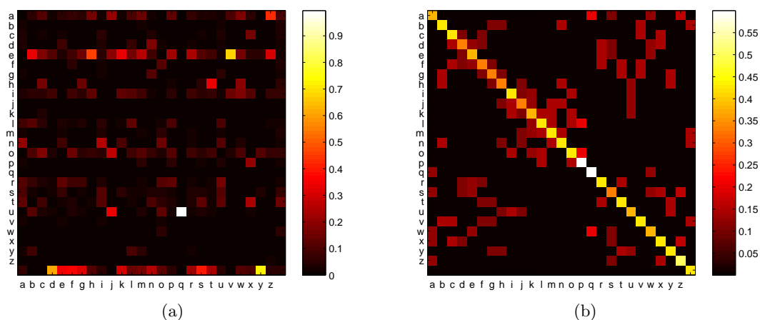
Figure 23.10: (a): The letter-to-letter transition matrix for English p(h' = i|h = j) . (b): The letter emission matrix for a typist with ‘stubby fingers’ in which the key or a neighbour on the keyboard is likely to be hit.
