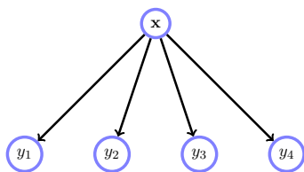
Figure 28.7: An information transfer problem. For a fixed distribution p(\mathbf{x}) and parameterised distributions p(y_j|\mathbf{x}) = \sigma(\mathbf{w}_i^T \mathbf{x}) , find the optimal parameters \mathbf{w}_i that maximise the mutual information between the variables \mathbf{x} and \mathbf{y} . Such considerations are popular in theoretical neuroscience and aim to understand how the receptive fields \mathbf{w}_i of a neuron relate to the statistics of the environment p(\mathbf{x}) .
