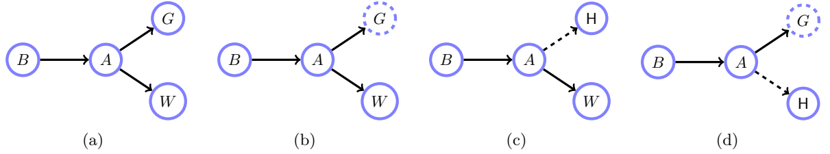
Figure 3.3: (a): Mr Holmes' burglary worries as given in [236]: (B)urglar, (A)larm, (W)atson, Mrs (G)ibbon. (b): Mrs Gibbon's uncertain evidence represented by a dashed circle. (c): Virtual evidence or the replacement of unreliable evidence can be represented by a dashed line. (d): Mrs Gibbon is uncertain in her evidence. Holmes also replaces the unreliable Watson with his own interpretation.
