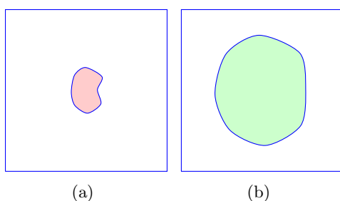
Figure 12.5: (a): The likelihood p(\mathcal{D}|\theta, M_{\text{complex}}) has a higher maximum value than then simpler model, but the likelihood drops quickly as we move away from regions of high likelihood. (b): The likelihood p(\mathcal{D}|\theta, M_{\text{simple}}) has a lower maximum value than then complex model, but the likelihood changes less quickly as we move away from regions of high likelihood. The corresponding volume of parameter space in which the model fits well can then be higher for the simpler model.
