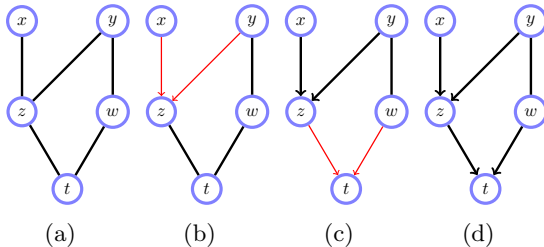
Figure 9.11: Skeleton orientation algorithm. (a) : The skeleton along with S_{x,y} = \emptyset , S_{x,w} = \emptyset , S_{z,w} = y , S_{x,t} = \{z, w\} , S_{y,t} = \{z, w\} . (b) : z \notin S_{x,y} , so form collider. (c) : t \notin S_{z,w} , so form collider. (d) : Final partially oriented DAG. The remaining edge may be oriented as desired, without violating the DAG condition. See also demoPCoracle.m .
