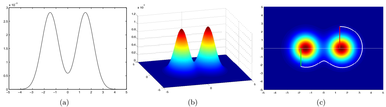
Figure 27.9: Hybrid Monte Carlo. (a) : Multi-modal distribution p(x) for which we desire samples. (b) : HMC forms the joint distribution p(x)p(y) where p(y) is Gaussian. (c) : This is a plot of (b) from above. Starting from the point x , we first draw a y from the Gaussian p(y) , giving a point (x, y) , given by the green line. Then we use Hamiltonian dynamics (white line) to traverse the distribution at roughly constant energy for a fixed number of steps, giving x', y' . We accept this point if H(x', y') > H(x, y') and make the new sample x' (red line). Otherwise this candidate is accepted with probability \exp(H(x', y') - H(x, y')) . If rejected the new sample x' is taken as a copy of x .
