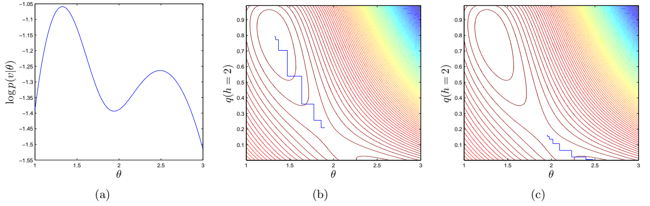
Figure 11.2: (a): The log likelihood for the model described in example(11.2). (b): Contours of the lower bound \tilde{L}(q(h=2), \theta) . For an initial choice \theta = 1.9 , successive updates of the E (vertical) and M (horizontal) steps are plotted, with the algorithm converging to the global optimum maximum likelihood setting for \theta . (c): Starting at \theta = 1.95 , the EM algorithm converges to a local optimum.
