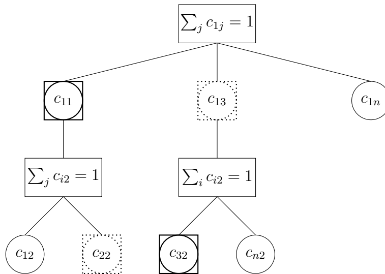
Figure 9.8: Tree for MWM problem.
