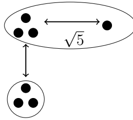
Figure 8.10: Example illustrating k -means does not satisfy the consistency axiom.
