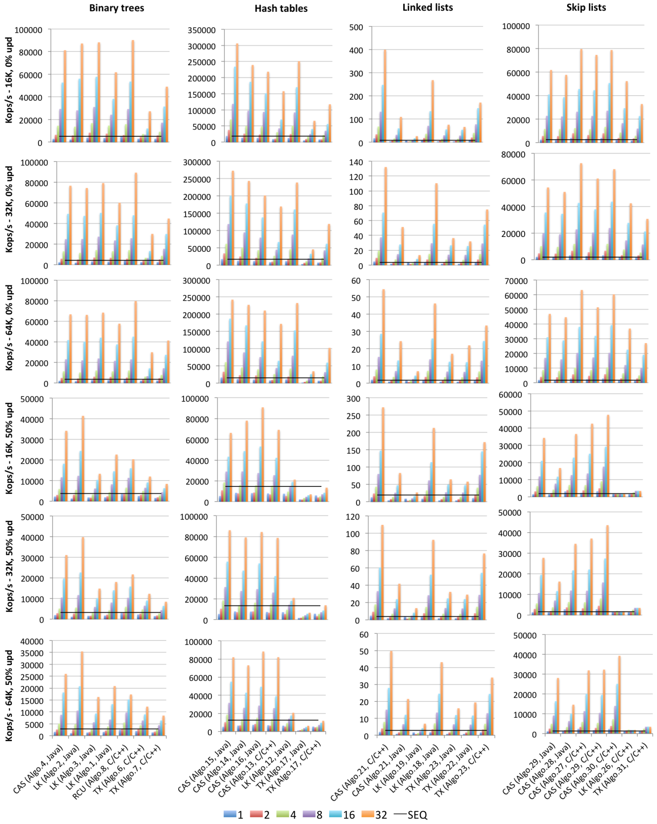
Figure 1. Synchrobench performance results for 1, 2, 4, 8, 16 and 32 threads on the 32-way Intel machine with data structures written in C/C++ and Java, and synchronized with read-modify-write (CAS), locks (LK), read-copy-update (RCU), and transactions (TX), and with sequential performance of non-synchronized data structures as the performance baseline (SEQ)
