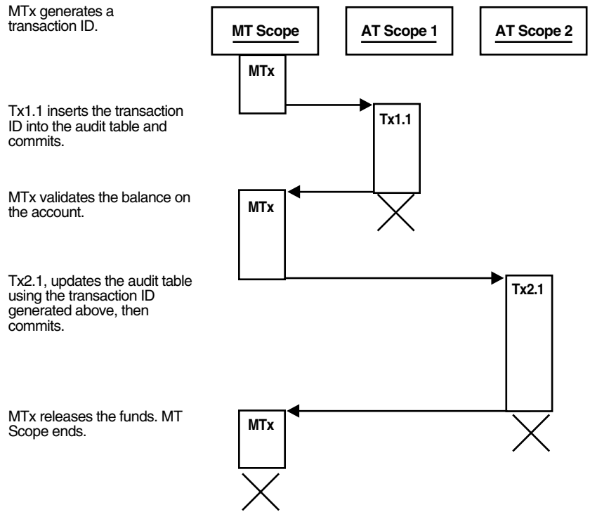
Figure 2–6 Bank Withdrawal—Sufficient Funds
