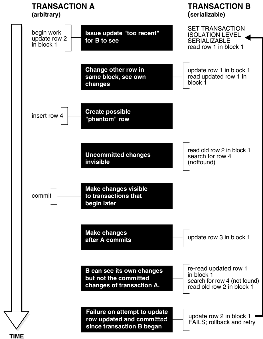
Figure 2–1 Interaction Between Serializable Transaction and Another Transaction
