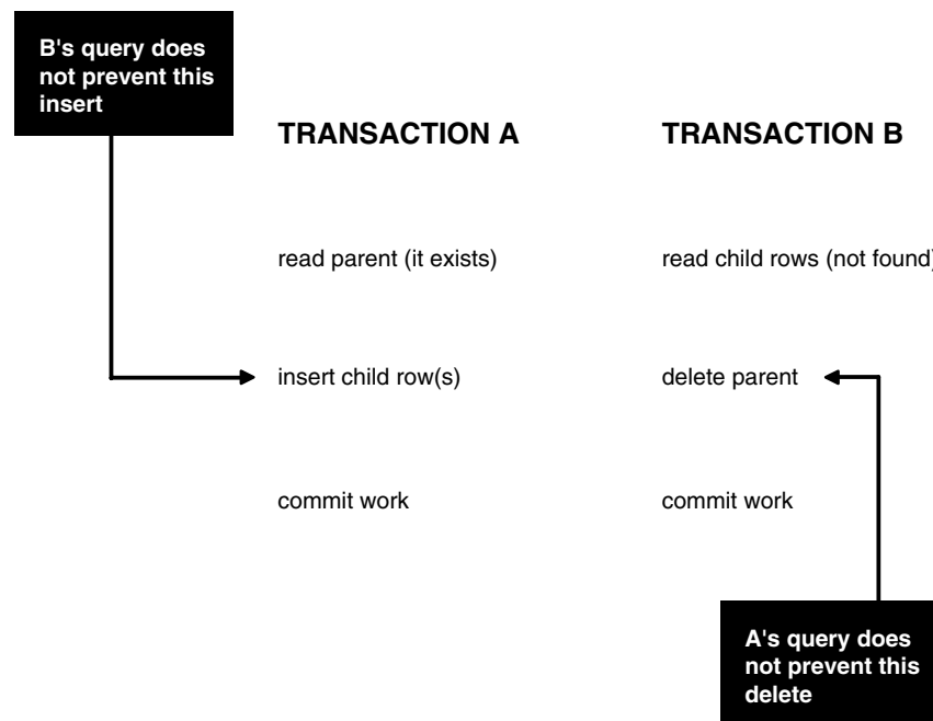
Figure 2-2 Referential Integrity Check
