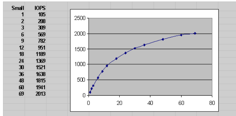
Figure 8–3 I/O Throughput at Different Small I/O Load Levels
