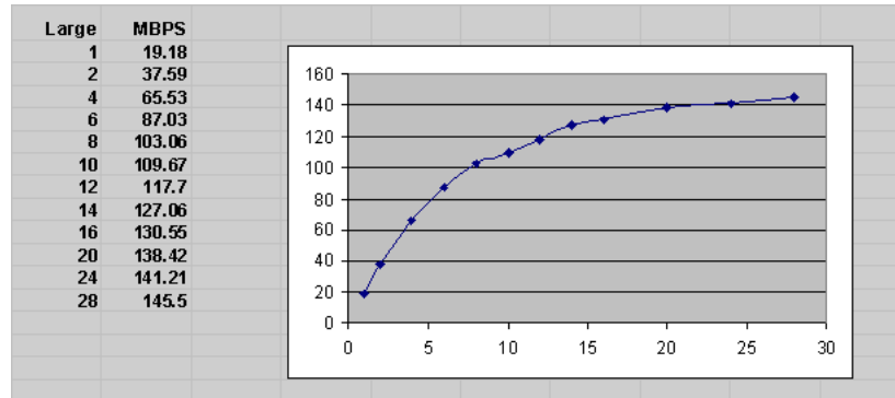
Figure 8–2 Sample I/O Load Levels
