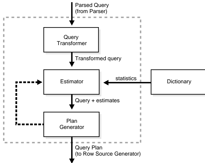
Figure 11–1 Optimizer Components
