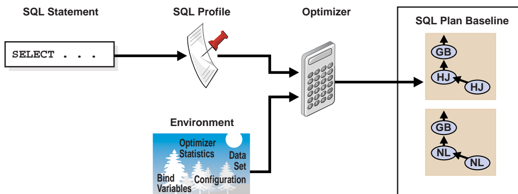
Figure 17-4 SQL Profile
