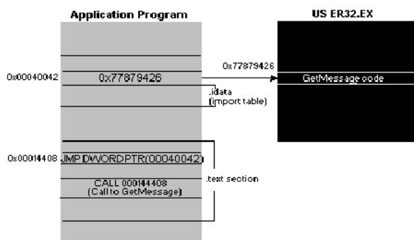
Figure 2. Calling a function in another module
