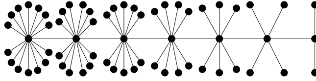
Figure 19.1: Distributed greedy algorithm: Bad example
