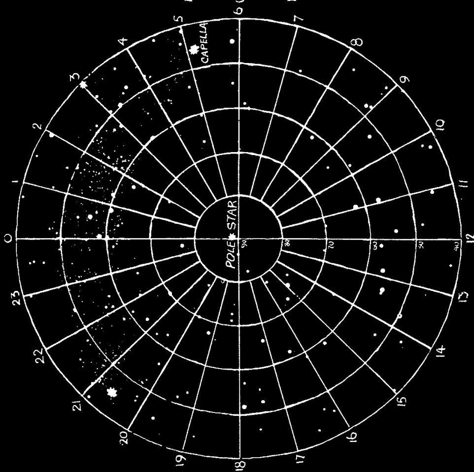
STAR POSITIONS - MIDNIGHT MARCH 21ST.
