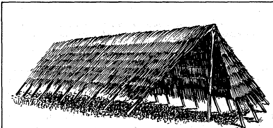
A finished long hut. Like the simple lean-to, this is basically a fine weather shelter. It has its origins in New Guinea and the Pacific Islands where, although the weather is often wet, it is not cold — hence the unthatched bottom to allow free air flow.
