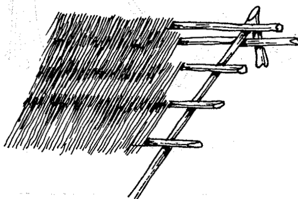
Assembly of thatching on a lean-to shelter. Note how the top frame projects forward and beyond the fork and the ridge itself to protect the front frame.
