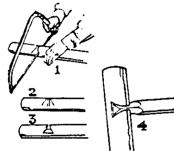
Figure 402 The Dove Tail Notch
