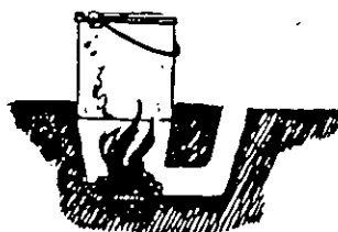
DAKOTA FIREPLACE IS WHITE MAN'S PRAIRIE FIRE FOR COOKING WITH A POT. "CHIMNEY" AT SIDE GIVES NECESSARY DRAFT.
