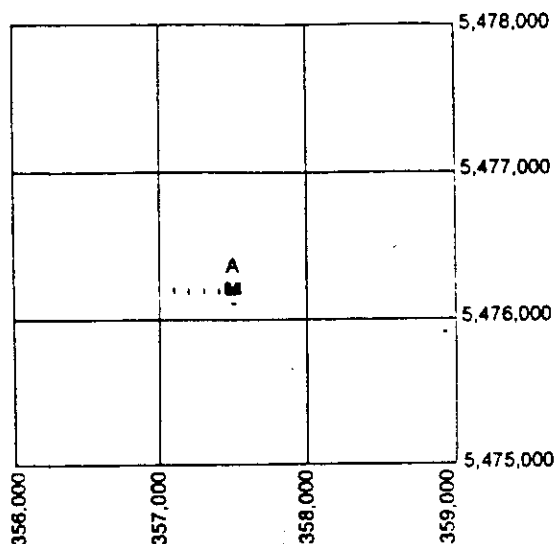
Figure 274 Reading a Map Reference
