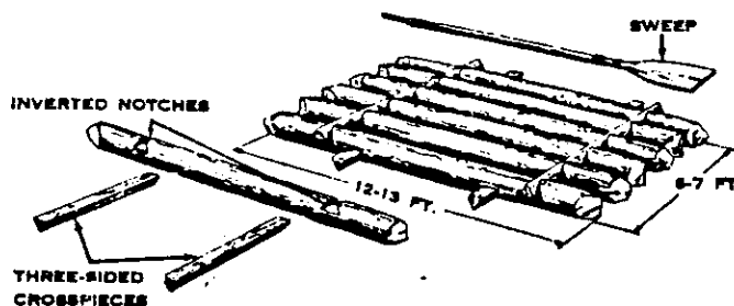
Figure 305 A Rugged Log Raft Developed by Northern Woodsmen
