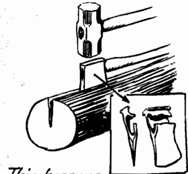
This happens when ax is used as a maul or a wedge!
