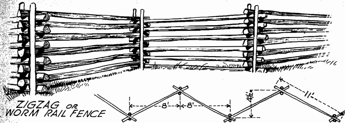
LOG FENCE
