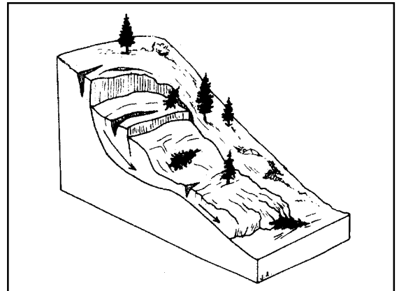
Figure 1. Diagrammatic sketch of a translational/rotational landslide. Drawing by Janet Appleby, Richard Kilbourne, and Thomas Spittler; modified from Varnes (1978).
